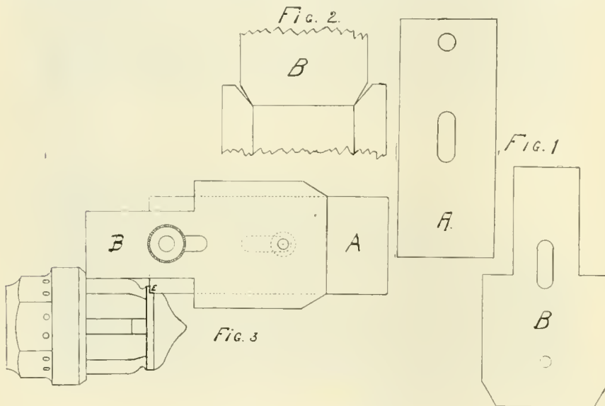
INSPIRATOR VALVE GAUGE.
